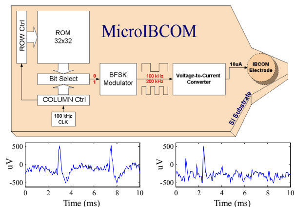
Fig. 3. Block Diagram of \mu -IBCOM showing the major CMOS circuit blocks and the different neural signals stored in \mu -IBCOM1 (left) and \mu -IBCOM2 (right)
